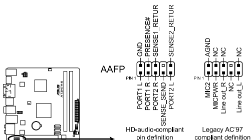
AT3N7A-I Analog front panel connector
